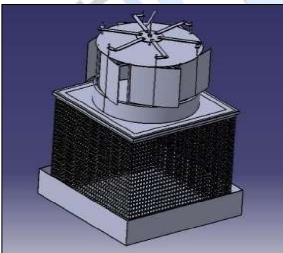
Figure 1. Air cooler with Cubical cooling chamber
